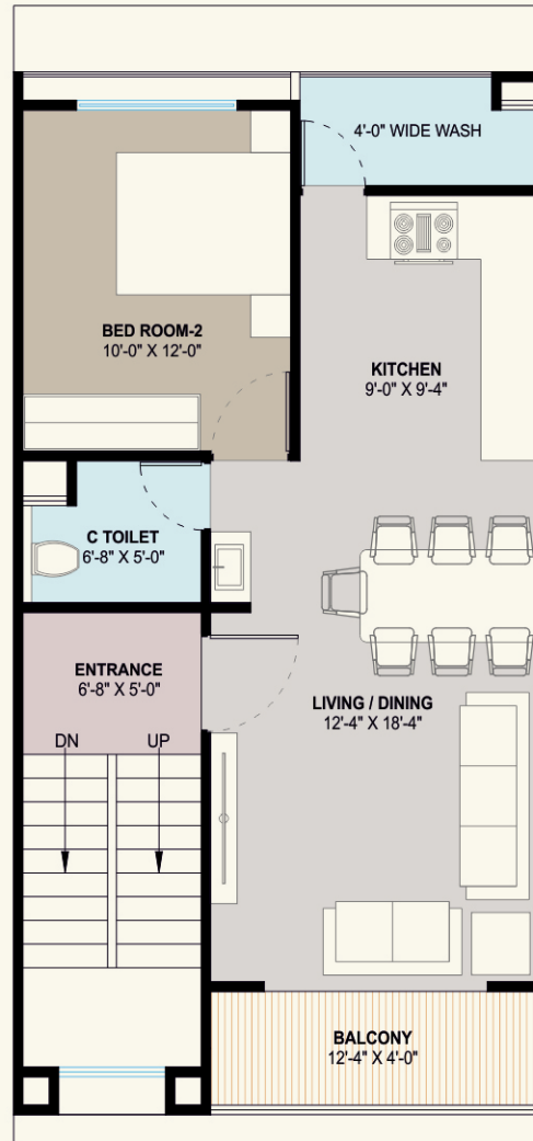
FIRST FLOOR
